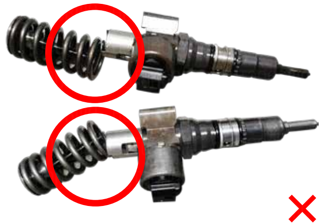
Loose spring
